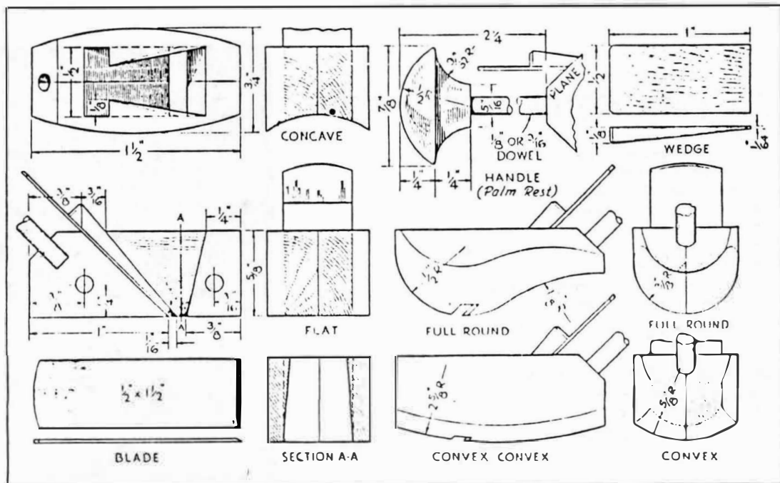
Full-size drawings of thumb planes to show the method of construction and various shapes found useful for models
