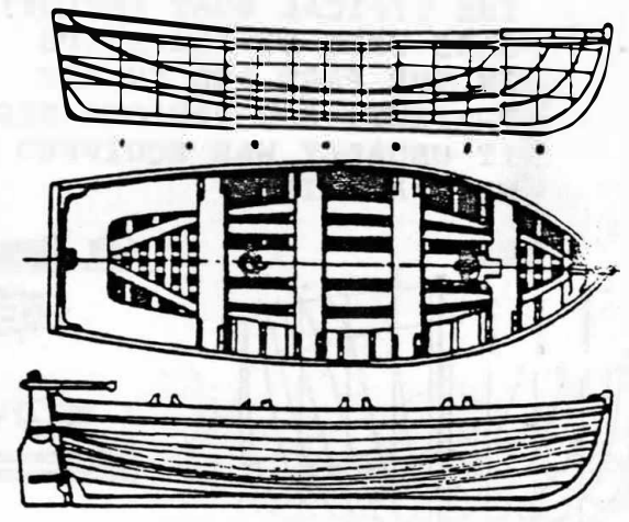
The row-boat on H.M.S. Victory
